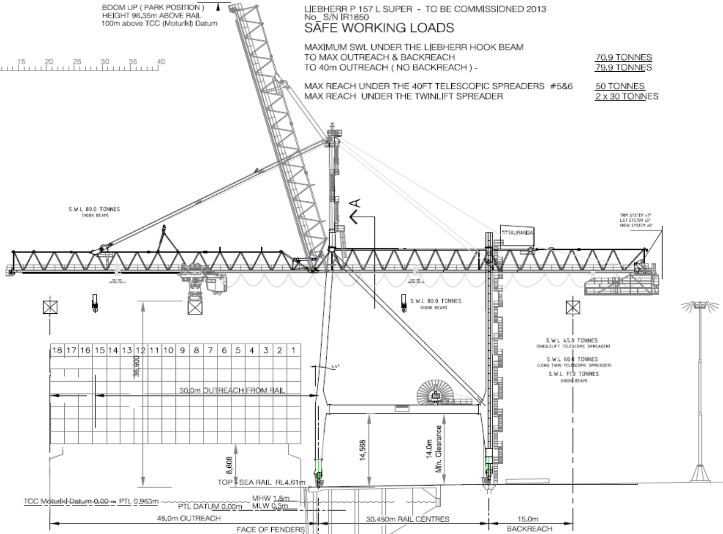
CRANE No.5 (6th) - LIEBHERR P 157 L SUPER IR1850 DIMENSIONS & LOADS
