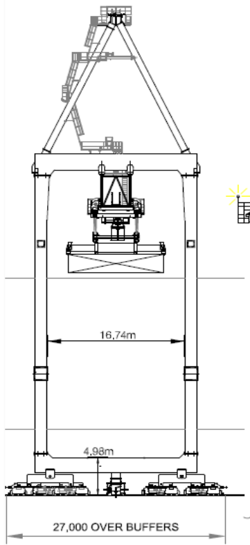
SECTION A-A LOOKING AT SHIP
