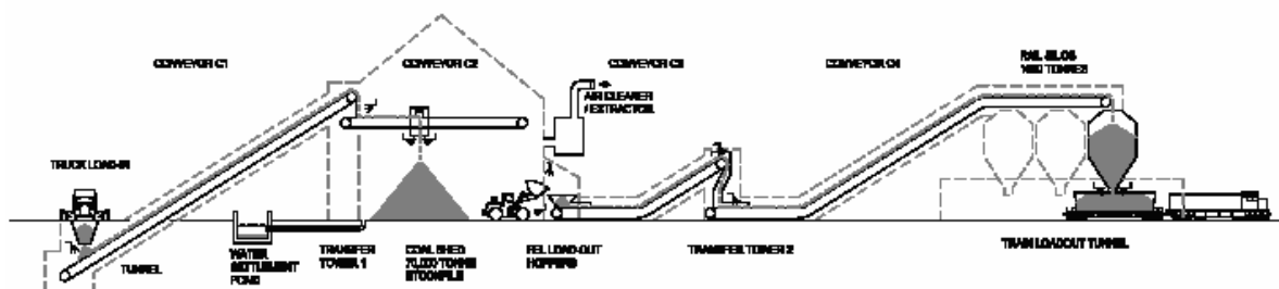
COAL FACILITY - DIAGRAMMATIC
