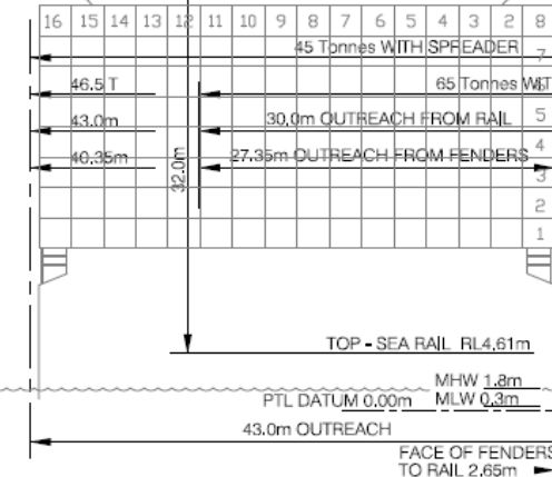
NORTH ELEVATION BERTHS 25,24,23
