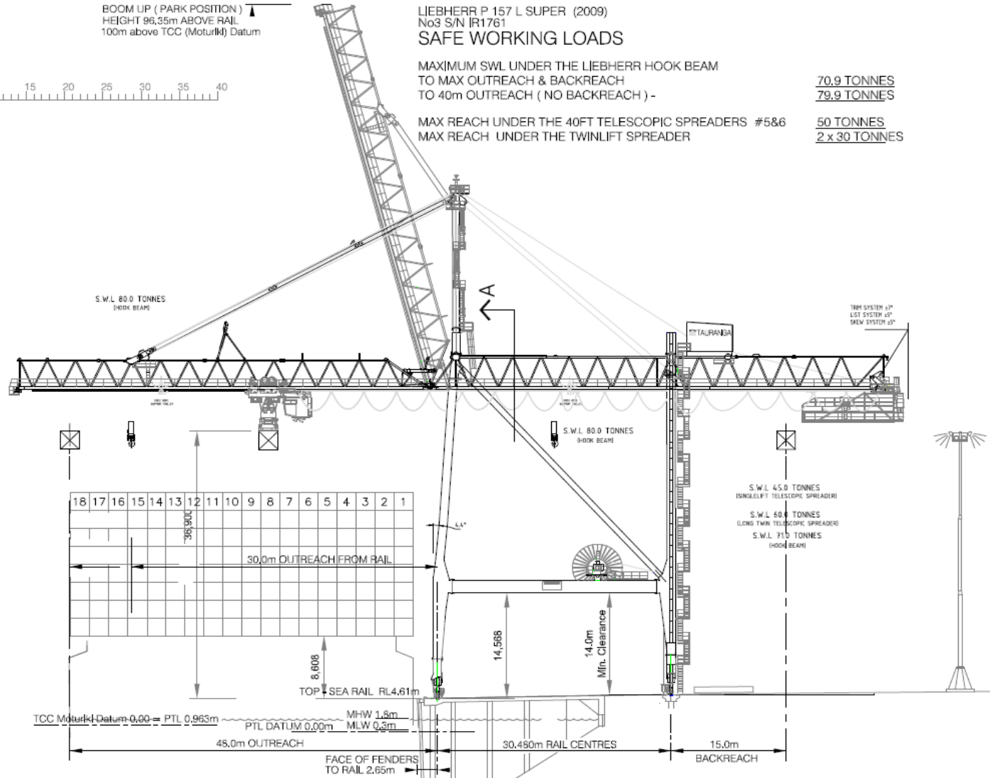
CRANE No.3 (5th) - LIEBHERR P 157 L SUPER IR1761 DIMENSIONS & LOADS
