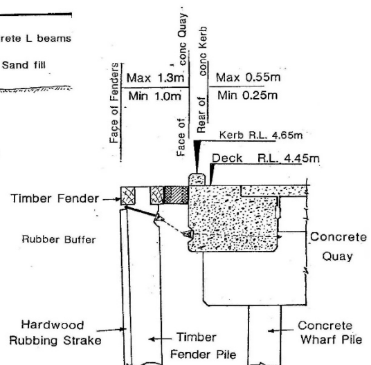
FENDER SYSTEM
