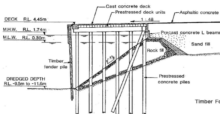
TYPICAL QUAY SECTION
