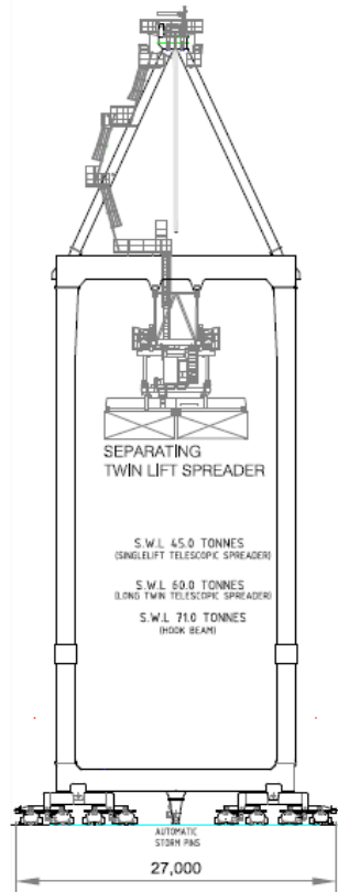
SECTION A-1
